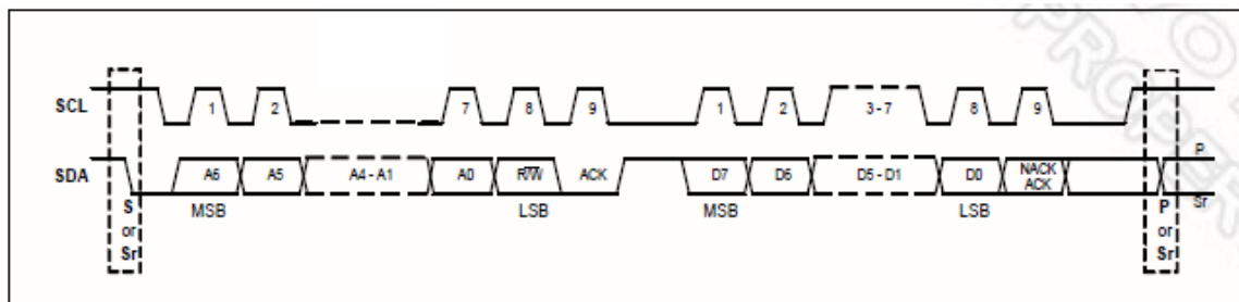
Figure 6-74 I 2 C Protocol
